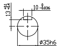
SHAFT EXTENSION
