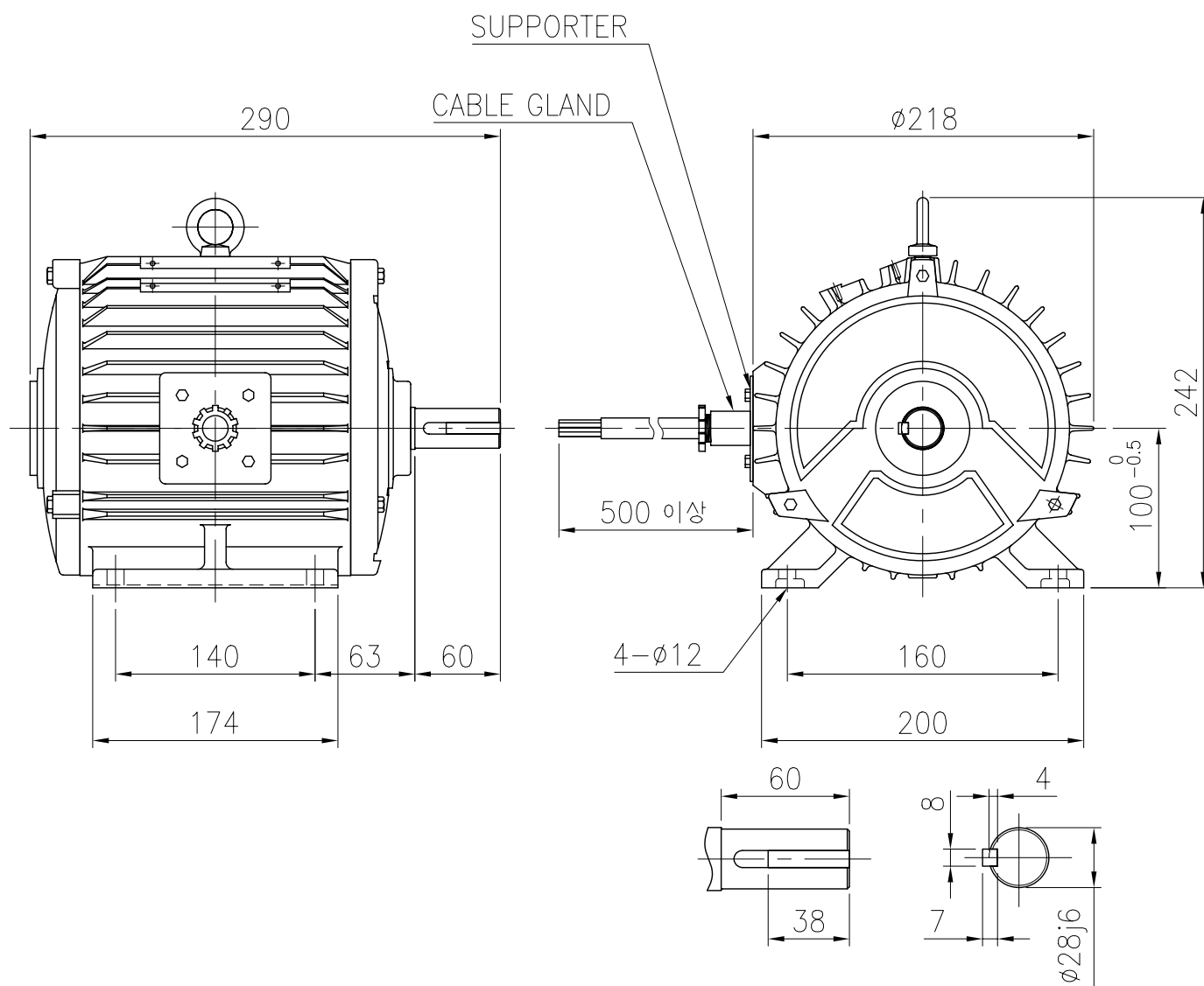
DETAIL OF SHAFT
